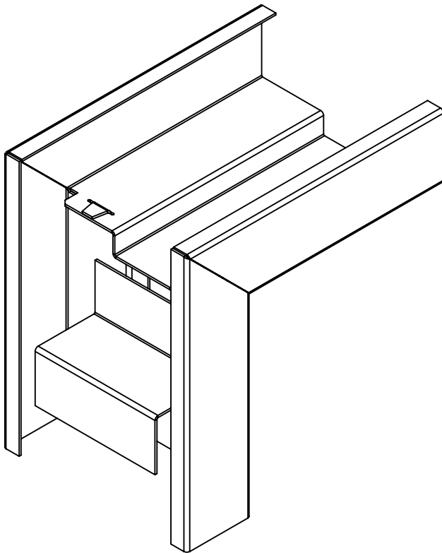
Flush Z Anchor
