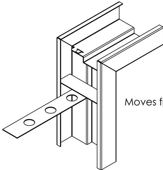
Loose T Anchor
