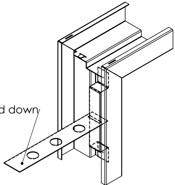
Welded T Anchor
