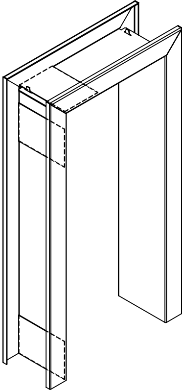
Single Acting Reinforcement
