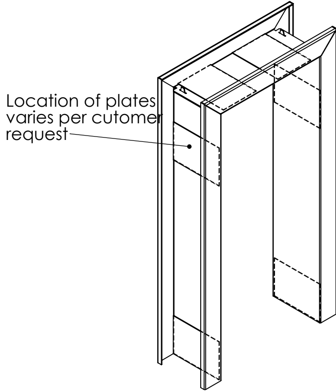
Double Acting Reinforcement
